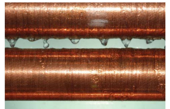
A falling-film evaporator is more efficient because refrigerant is sprayed over the tubes, offering improved heat transfer and reducing refrigerant charge by 30%.
