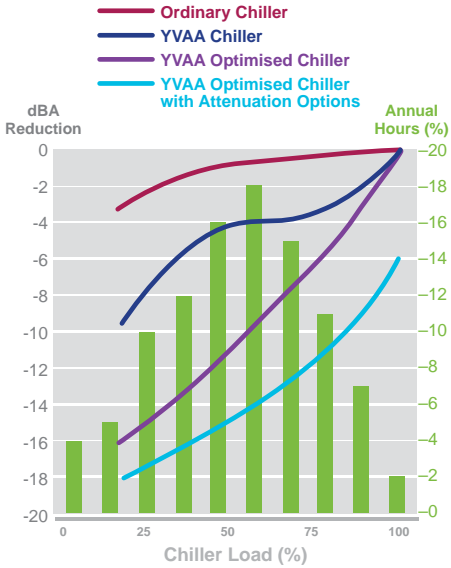
An optimised YVAA chiller can reduce ambient noise by as much as 16 dBA.
